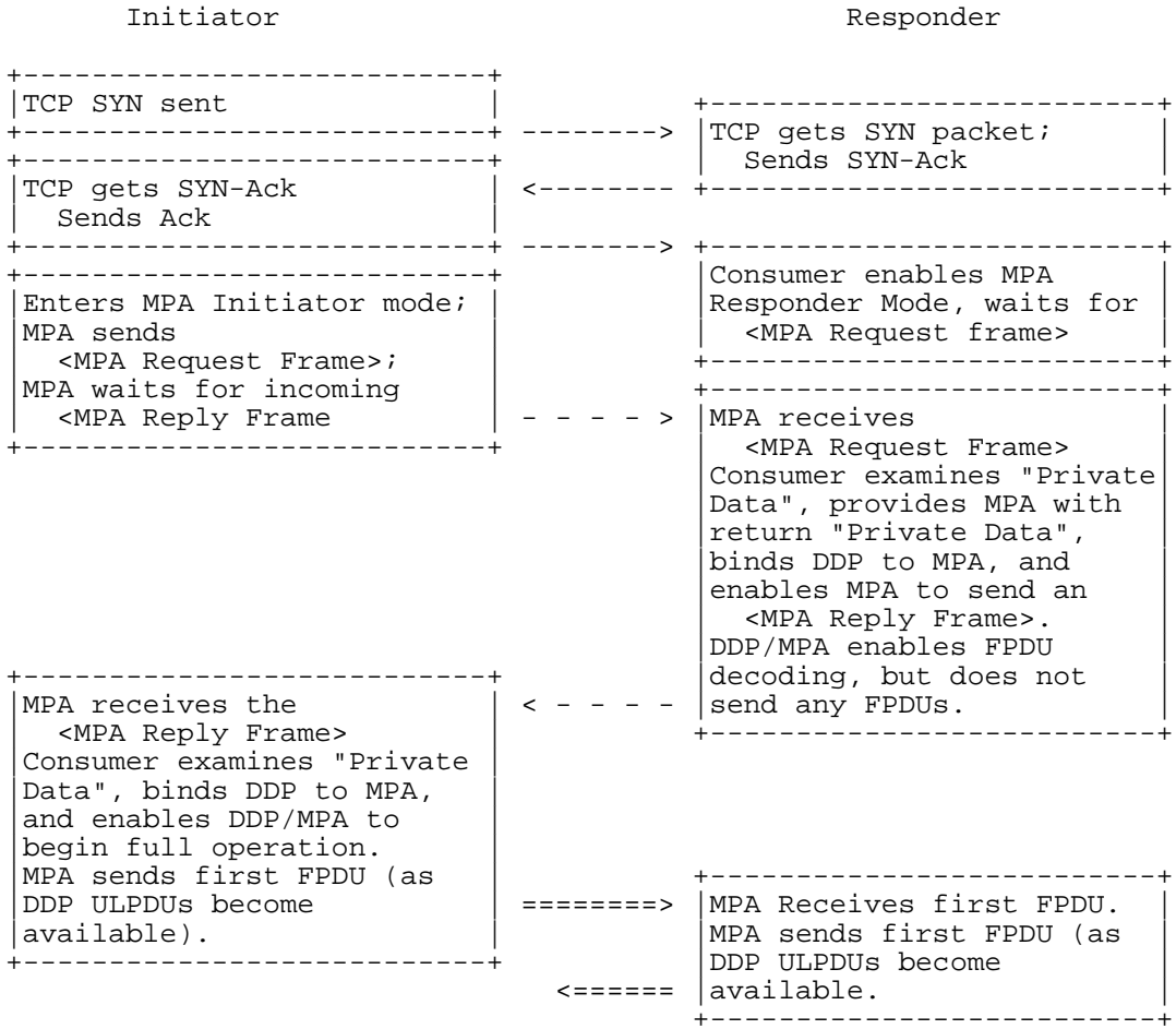
Figure 9: Example Immediate Startup negotiation
