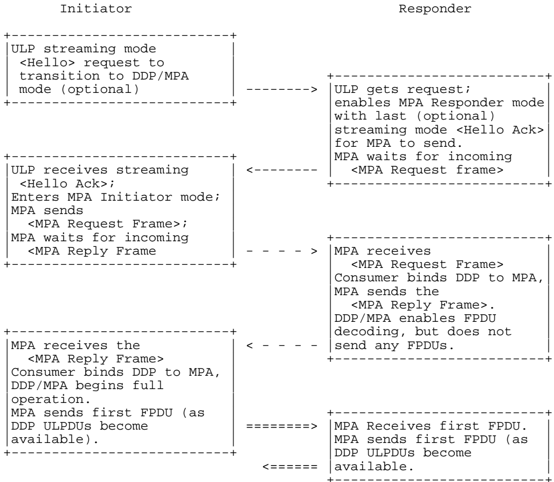
Figure 8: Example Delayed Startup negotiation
