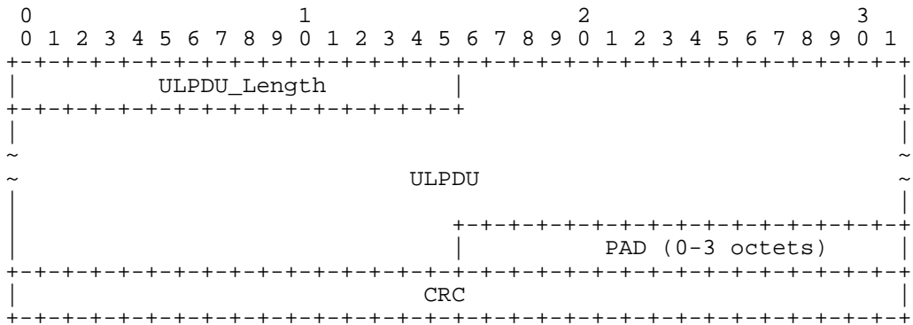
Figure 2 FPDU Format
