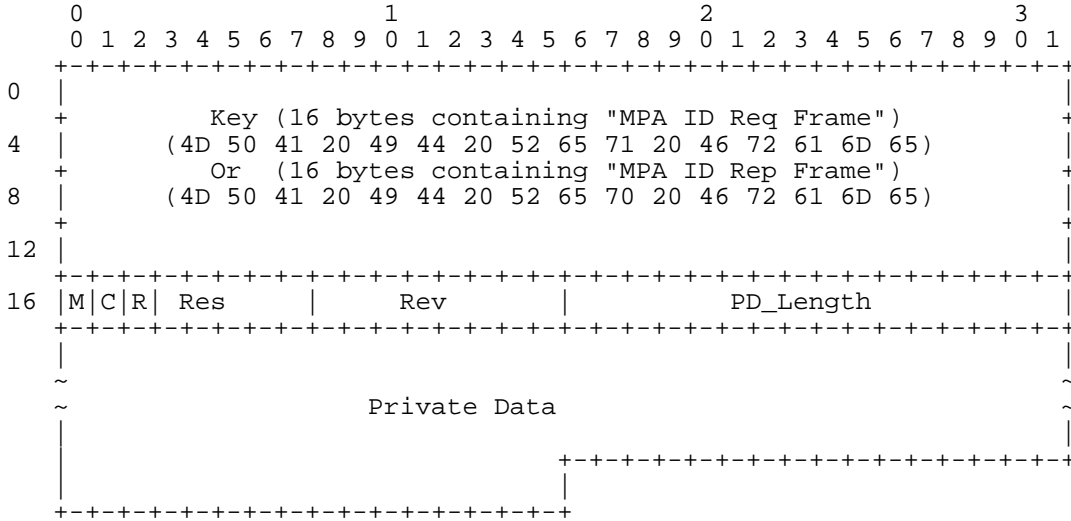
Figure 7 "MPA Request/Reply Frame"
