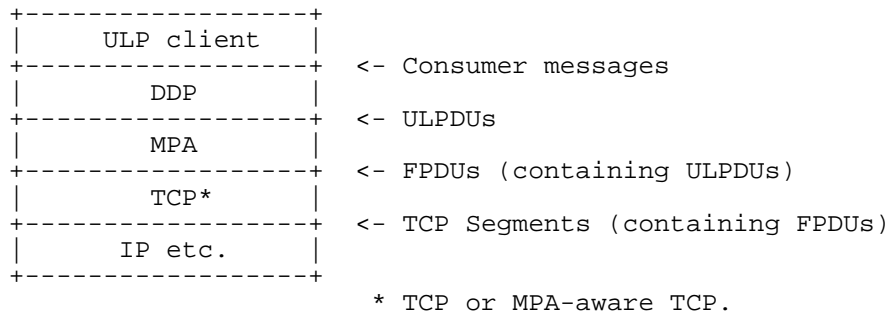
Figure 1 ULP MPA TCP Layering
