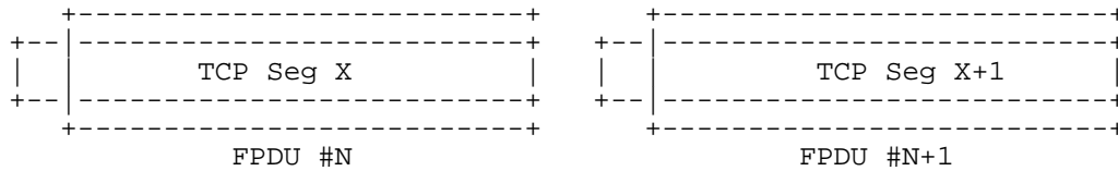
Figure 11: Aligned FPDU placed immediately after TCP header
