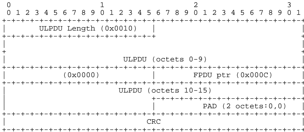
Figure 4 Example FPDU Format with Marker
